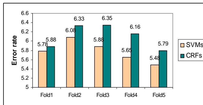
Fig. 2. Performance comparison between CRFs (SC + VSD + Dict) and SVMs on 5-fold CV test
