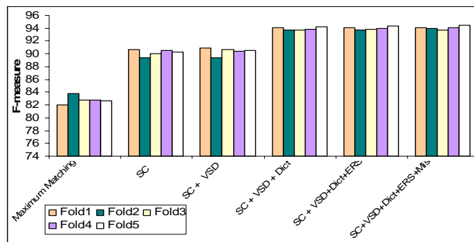
Fig. 1. Performance comparison among CRF models using different feature settings (Maximum Matching as the baseline)
